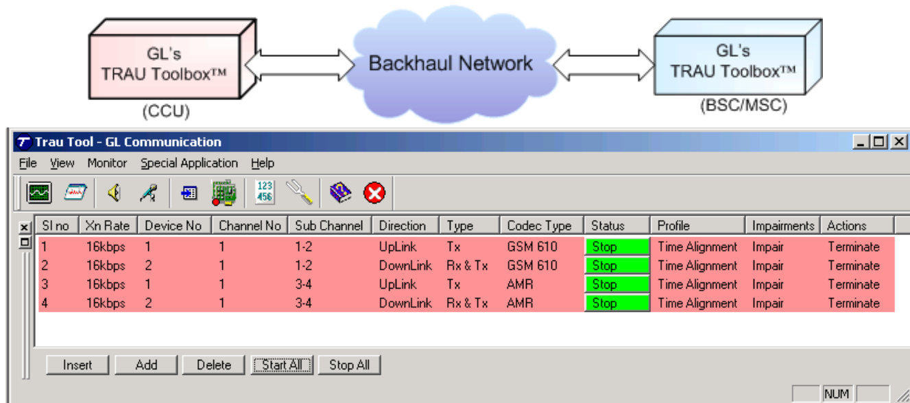
Figure: TRAU ToolBox™
