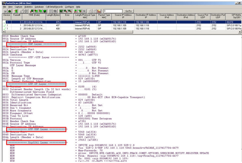
Figure: Detail View of VoLTE
