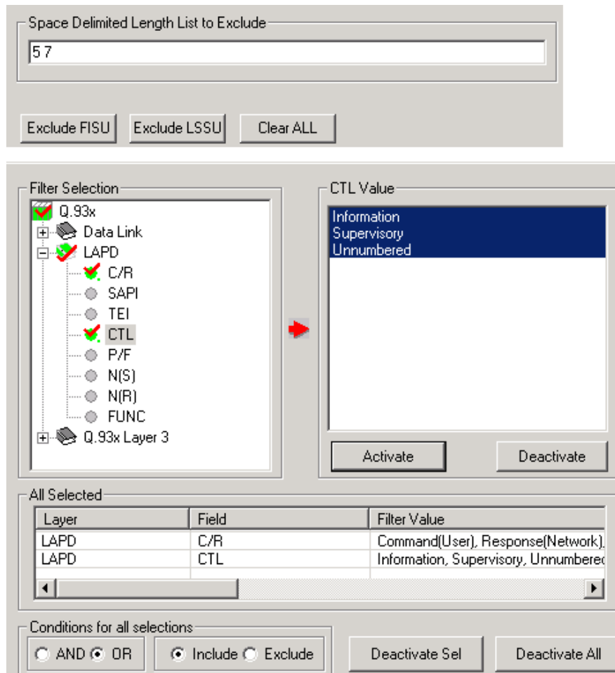
Figure: Real-time and Offline Filter
