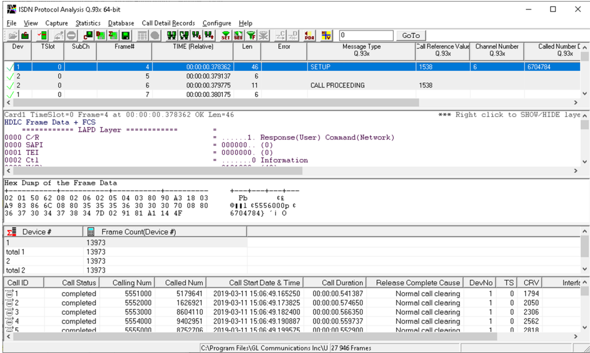
Figure: Summary, Detail, and Hex dump Views
