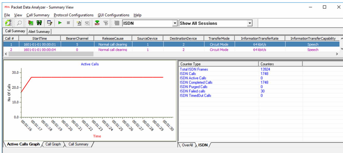
Figure: Call Capture Option with PDA
