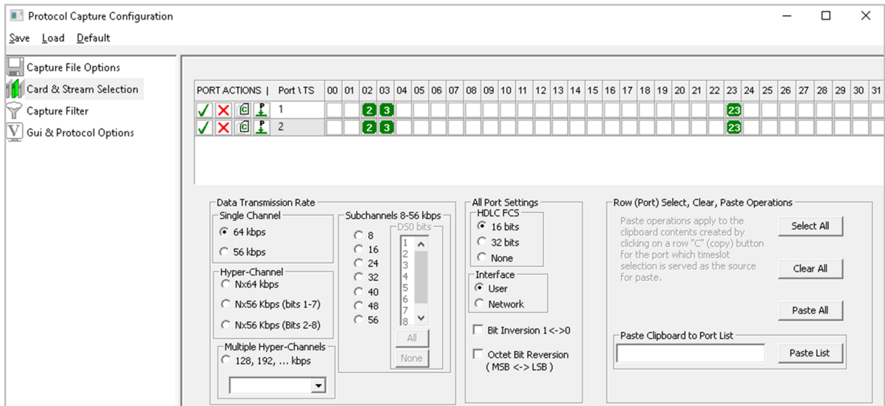
Figure: Stream / Interface Selection
